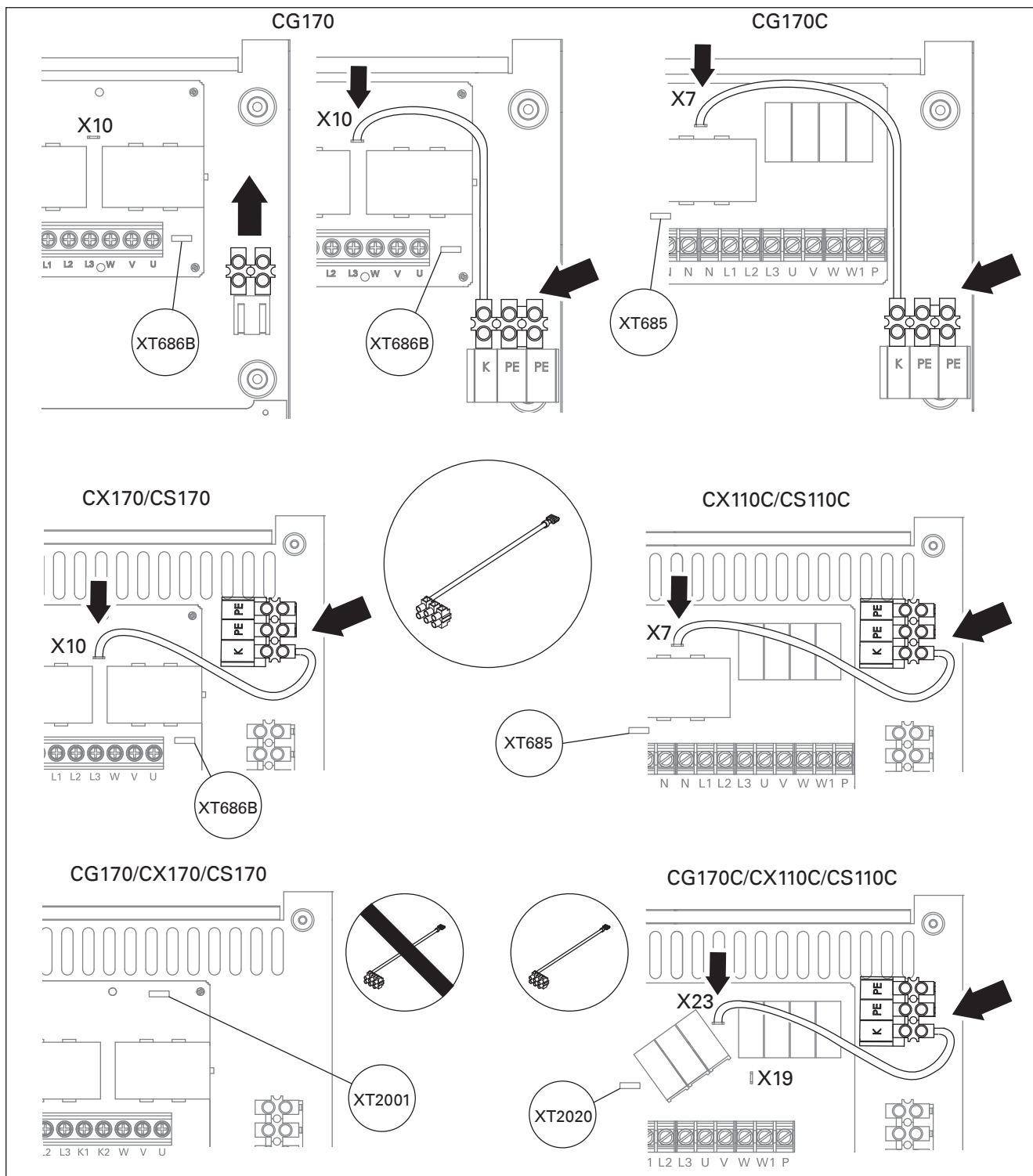
Figure 4. Connection of additional terminal block inside the power unit CG170/CG170C/CX170/CX110C/CS170/CS110C
