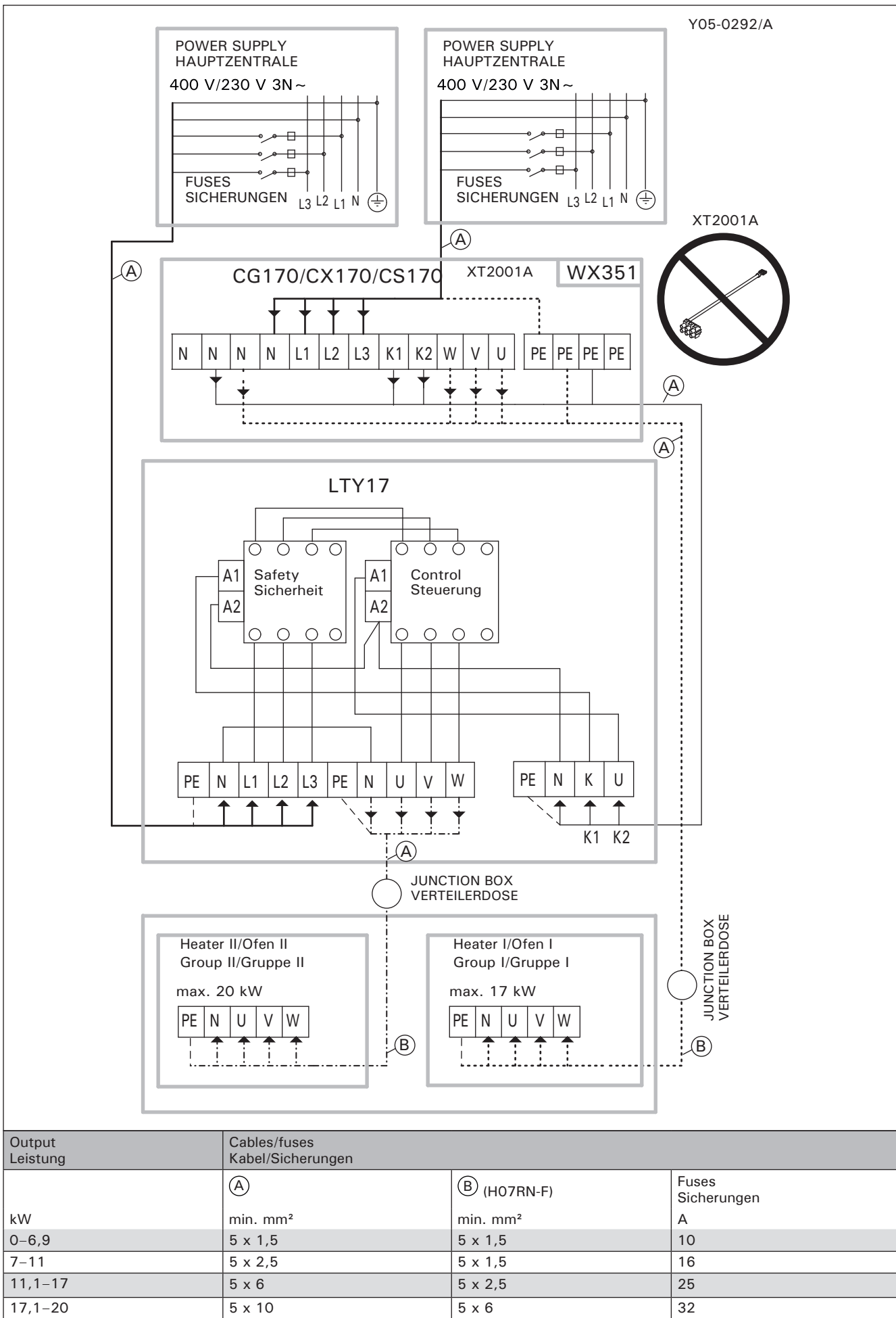
Figure 7. Connection of power extension unit LTY17 with control unit CG170, CX170 or CS170 (XT2001A).
